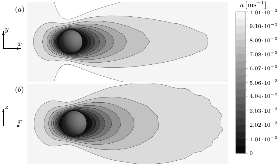
Fig. 3. The velocity wake in (a) an xy -plane perpendicular and (b) an xz -plane parallel to the magnetic field. A distinct asymmetry, with a preference for a velocity spread along the field lines, can be seen behind the sphere. A characteristic dent in the velocity contours can be observed near the sides of the sphere. This is due to the electric field the volume charges here add to \mathbf{E}_0 , which increases the electric current in the y -direction and thereby increases the accelerating Lorentz force.
