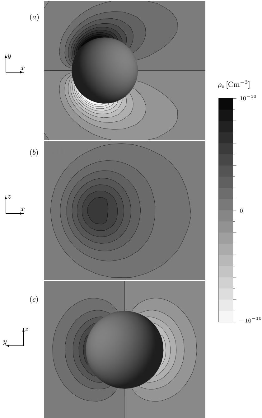
Fig. 6. The volume charge density \rho_e in (a) the xy -plane, (b) the xz -plane touching the side of the sphere and (c) the yz -plane for Re = 10 and Ha = 2 .
