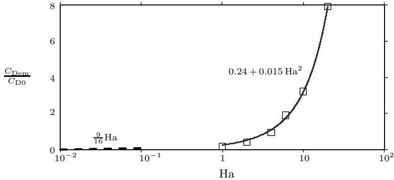
Fig. 13. The analytical result for the relative electromagnetic drag C_{Dem}/C_{D0} for Ha , Re \ll 1 [8] is extended with simulations to 1 \leq Ha \leq 20 .
